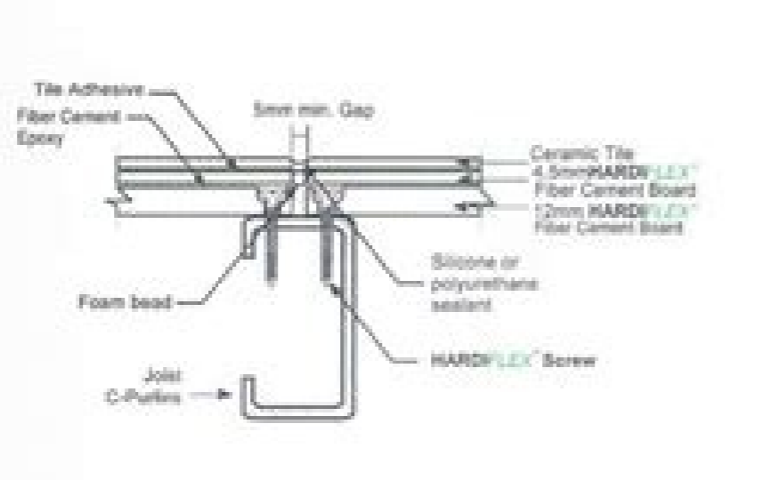
Figure 19 Control Joint
